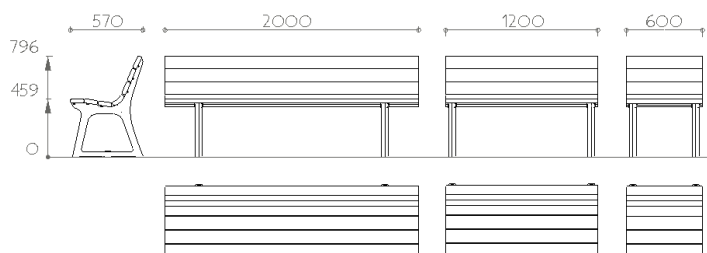
Banc 3 places
